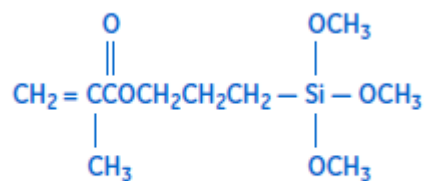
Gamma-Methacryloxypropyltrimethoxy Silane
